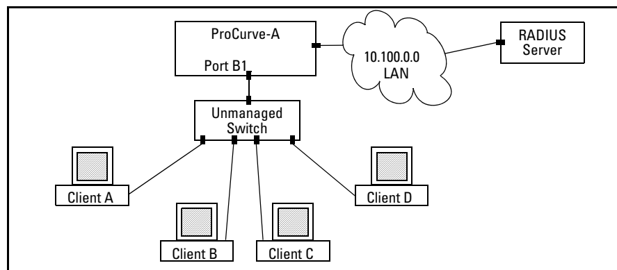
Figure 9-1. Example of Multiple Clients Authenticating Through a Single Port
